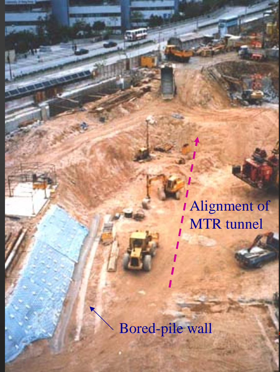
Protecting the MTR tunnel by forming a cut-off bored-pile wall on the sides
