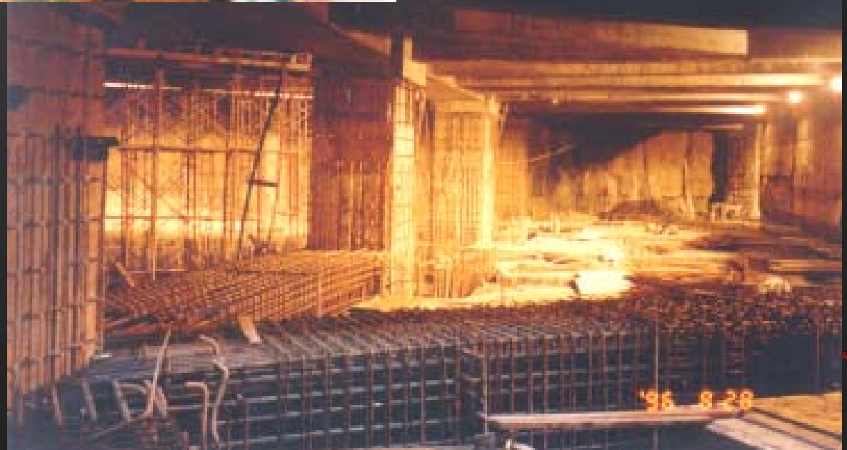
Forming the ground beams at the formation level of the lowest basement level
